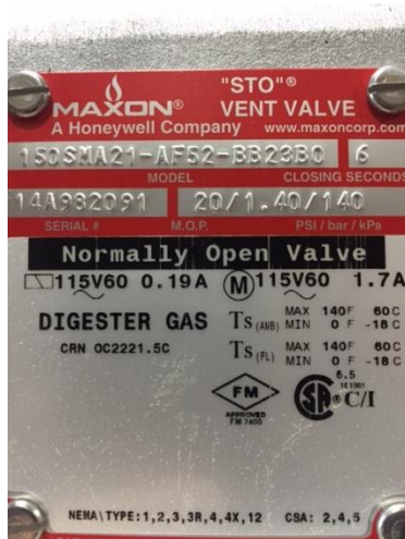
Valve #2
