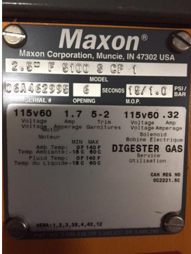
Valve #1
